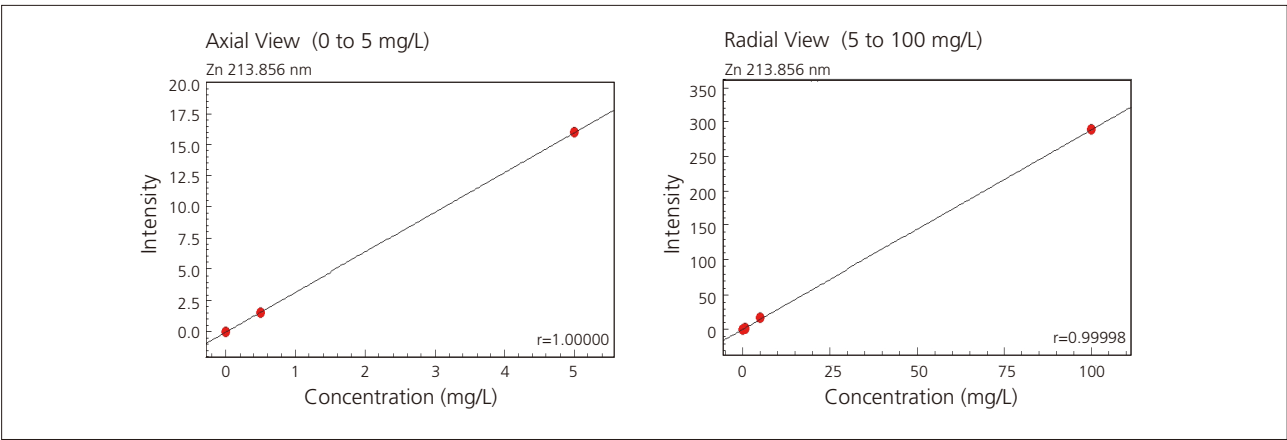
Fig. 1 Calibration Curves of Zn by Axial View and Radial View
