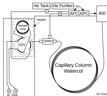
Fig. 1 Trace Moisture Analysis System
