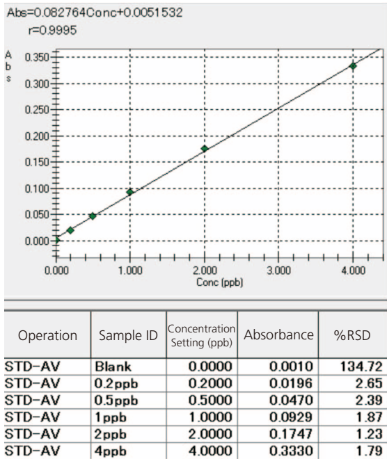
Fig. 2 Calibration Curve for As
