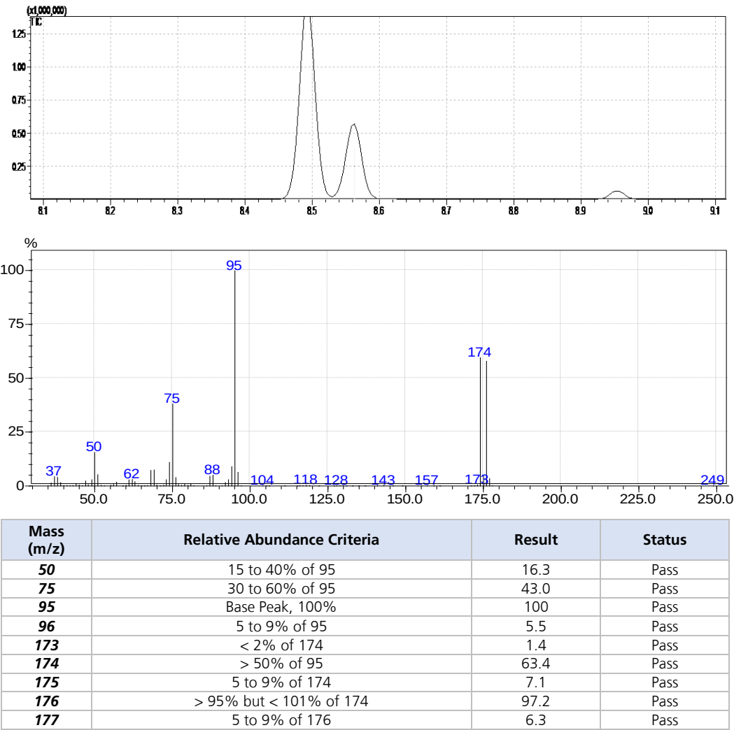
Figure 2: Typical Results from BFB Tune Evaluation Using US EPA Method 624 Criteria
