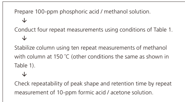
Fig. 3 Procedure for Column Phosphoric Acid Treatment
