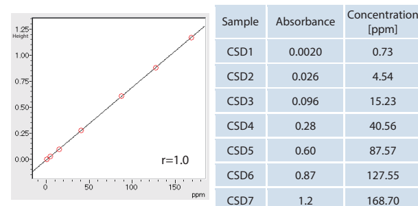
Fig. 3 Calibration Curve and Standard Sample Concentrations
