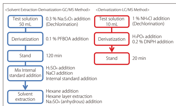
Fig. 1 Pretreatment Work Flows
