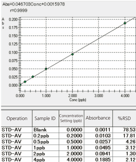
Fig. 3 Calibration Curve for Se
